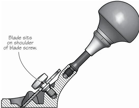
Figure 4: Blade clamping.
